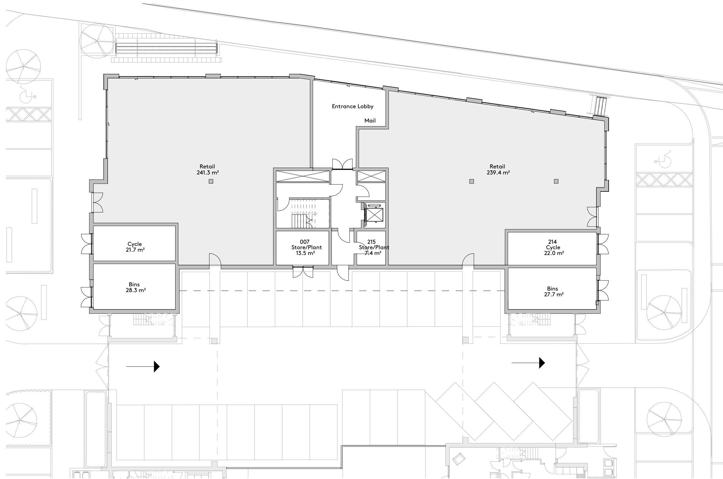
Block D Ground Floor 1 : 200
